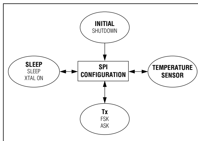
Figure 11. Operating Modes
