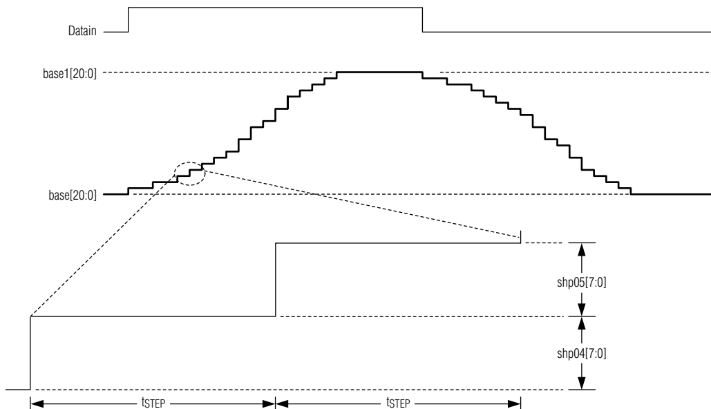
Figure 17. Tx FSK Frequency Waveshaping Timing Diagram
