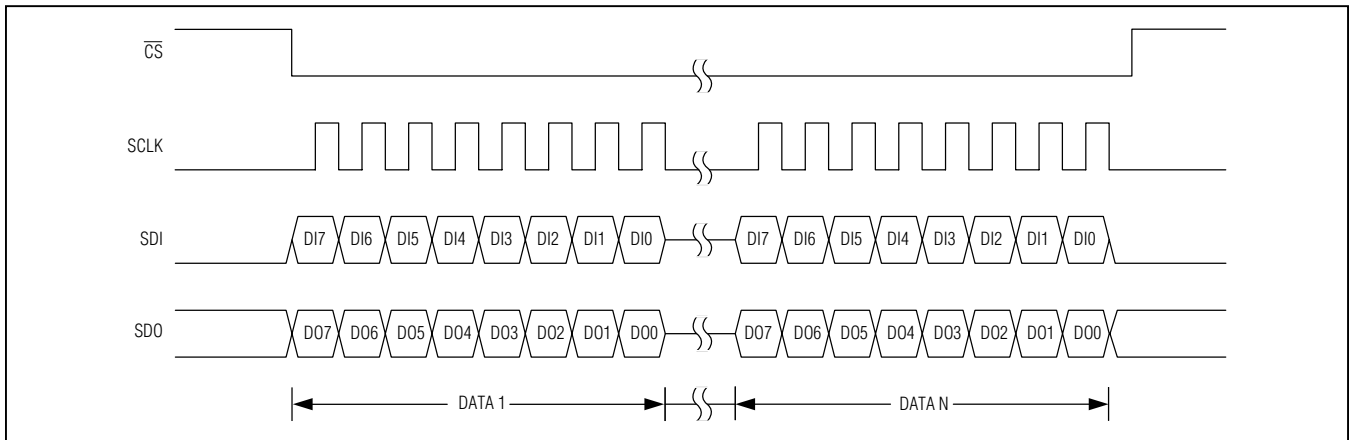
Figure 6. SPI Format
